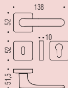
CC21 R-RY 52X52
