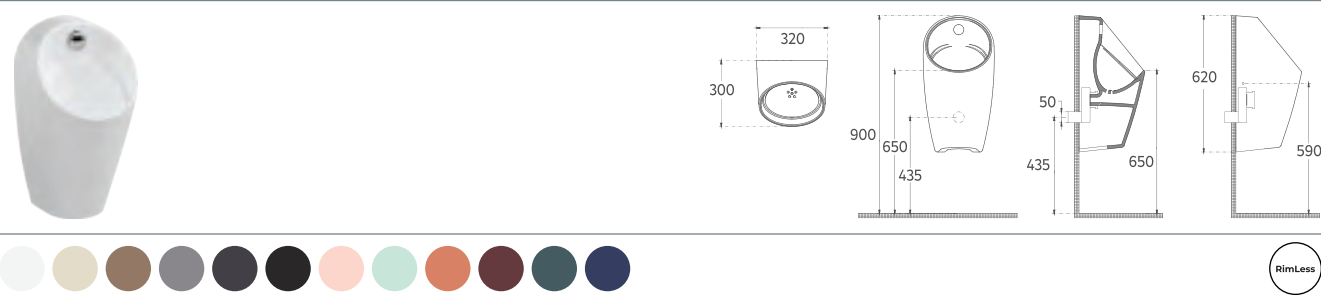
10NFS92001 SensoClean Urinal
