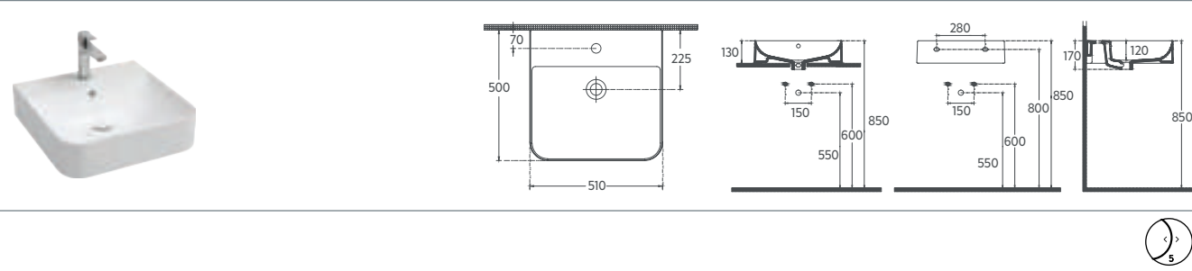
SOTT’AQUA Countertop Washbasin, 51 cm
