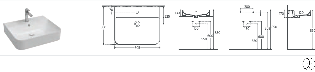
SOTT’AQUA Countertop Washbasin, 61 cm
