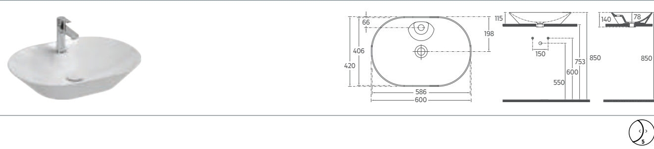
SISTEMA Y Countertop Washbasin, 60 cm
