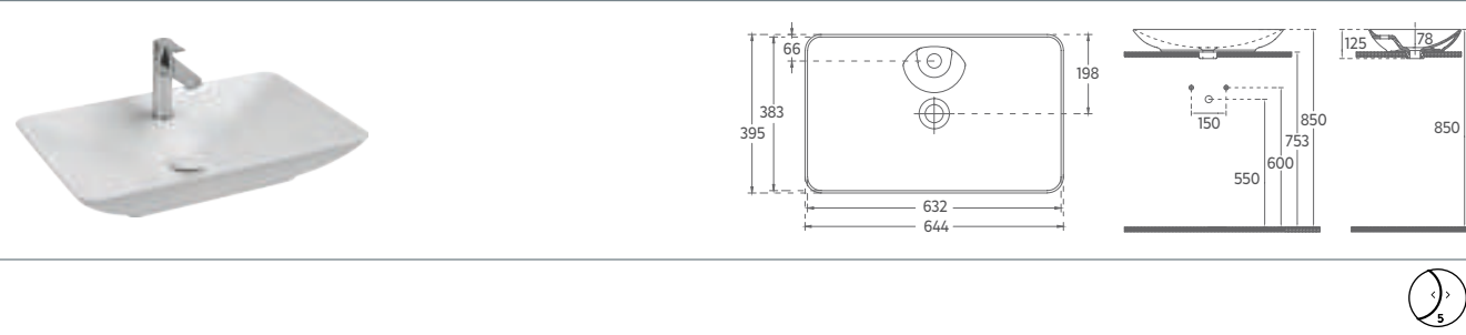
SISTEMA Y Countertop Washbasin, 65 cm
