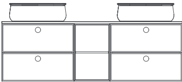
COUNTERTOP DOUBLE DRAWER WASHBASIN UNIT
