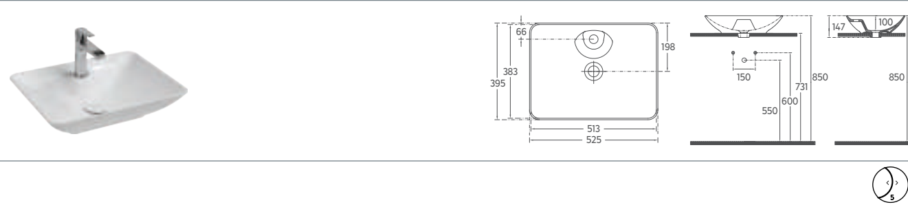
SISTEMA Y Countertop Washbasin, 52 cm
