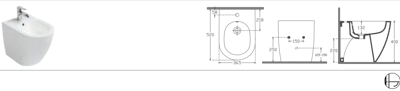
10NF42001 Floor Standing Bidet
