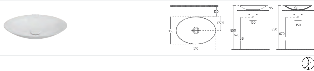
SISTEMA Y Countertop Washbasin, 51 cm
